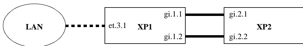
Figure 6. Configuring per VLAN spanning tree with RSTP enabled
