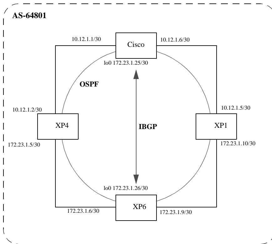
Figure 12. Sample IBGP Configuration (Routing Group Type)
