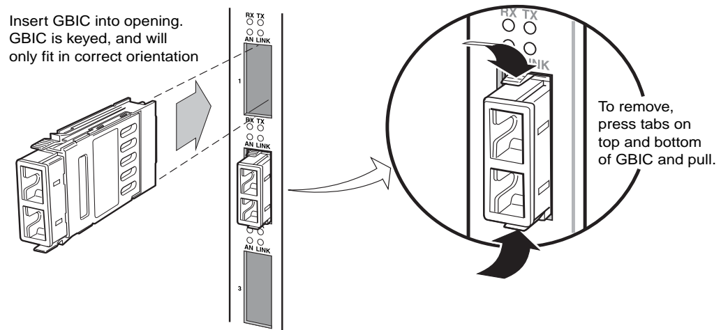
Figure 5. Installing and removing a GBIC.
