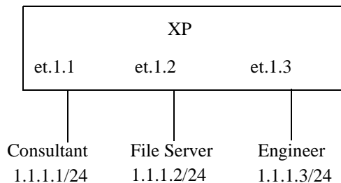
Figure 27. Sample VLAN for Layer-4 bridging
