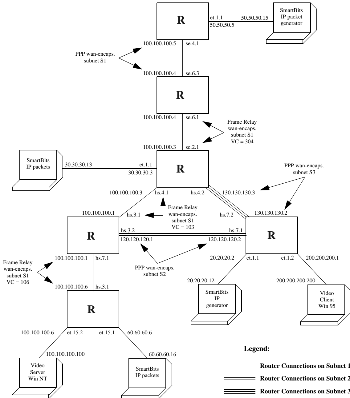
Figure 30. Multi-router WAN configuration
