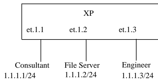
Figure 26. Sample VLAN for Layer-4 bridging
