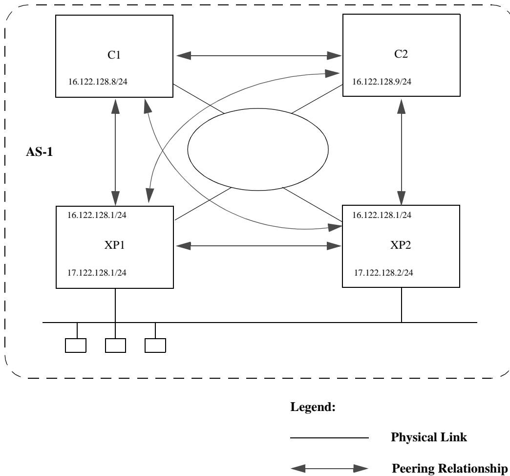
Figure 12. Sample IBGP Configuration (Internal Group Type)
