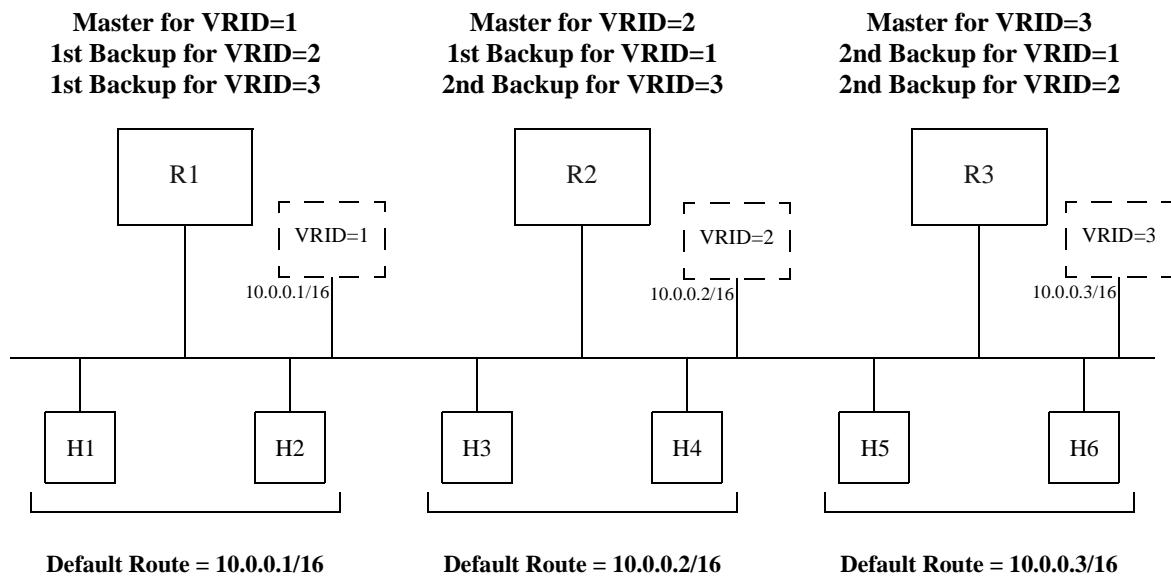
Figure 8. Multi-Backup VRRP Configuration
