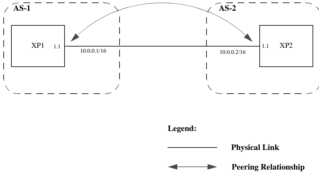
Figure 10. Sample BGP Peering Session
