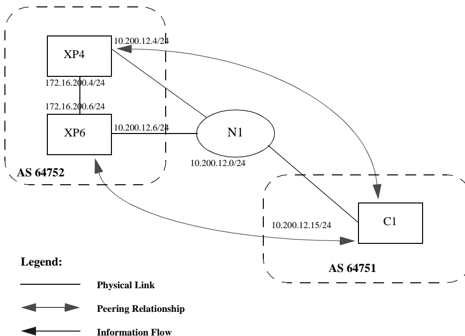
Figure 16. Sample BGP Configuration (MED Attribute)
