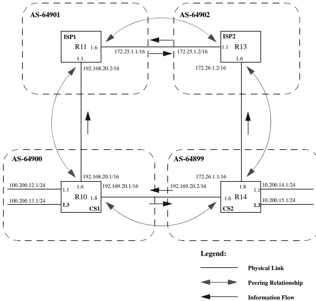
Figure 13. Sample BGP Configuration (Specific Community)
