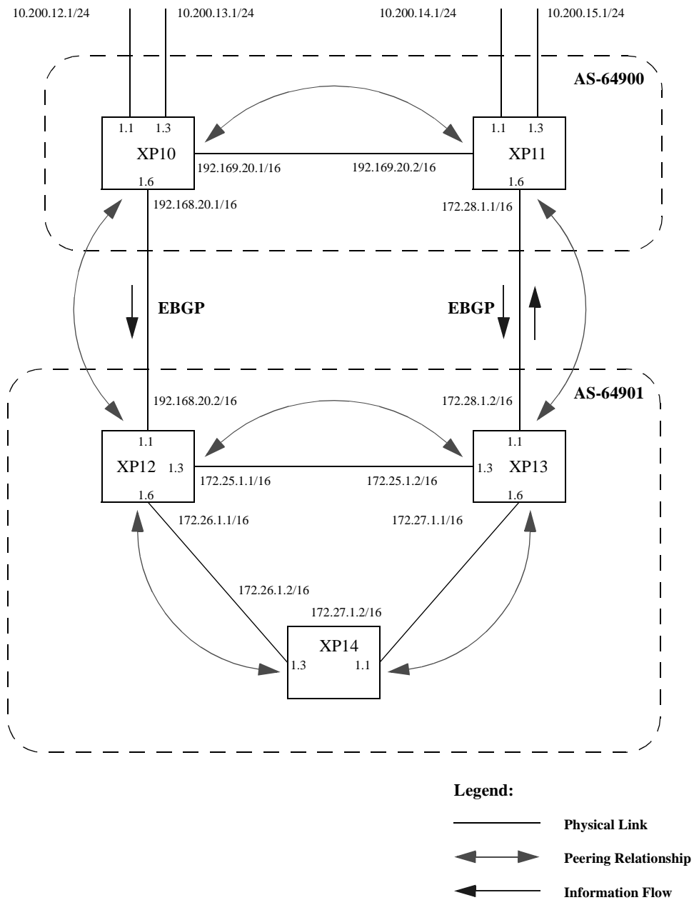
Figure 15. Sample BGP Configuration (Local Preference)
