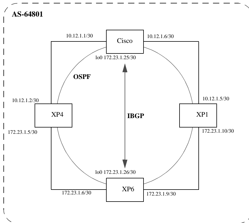
Figure 11. Sample IBGP Configuration (Routing Group Type)
