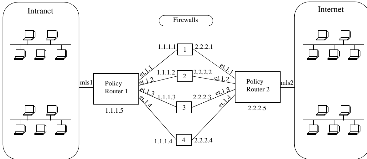
Figure 24. Selecting Next Hop Gateway from IP Packet Information
