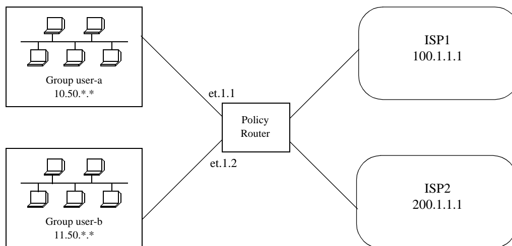
Figure 21. Using an IP Policy to Route Traffic to Two Different ISPs
