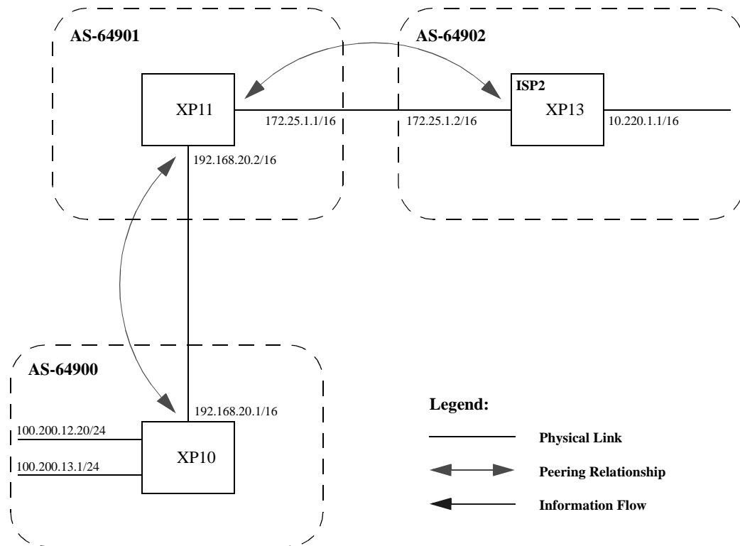
Figure 14. Sample BGP Configuration (Well-Known Community)
