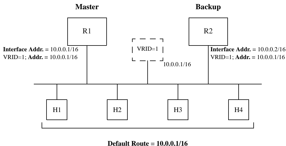
Figure 6. Basic VRRP Configuration
