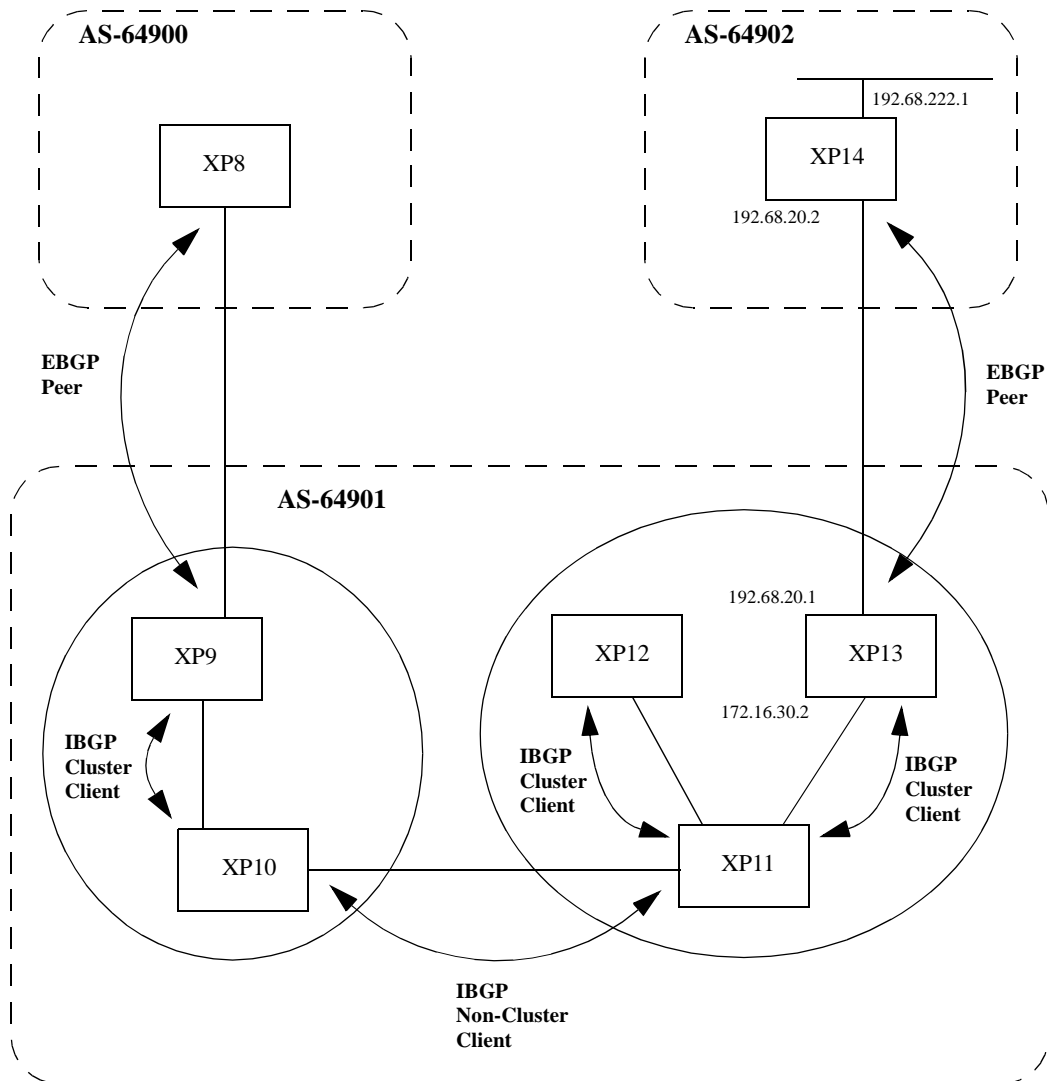
Figure 18. Sample BGP Configuration (Route Reflection)
