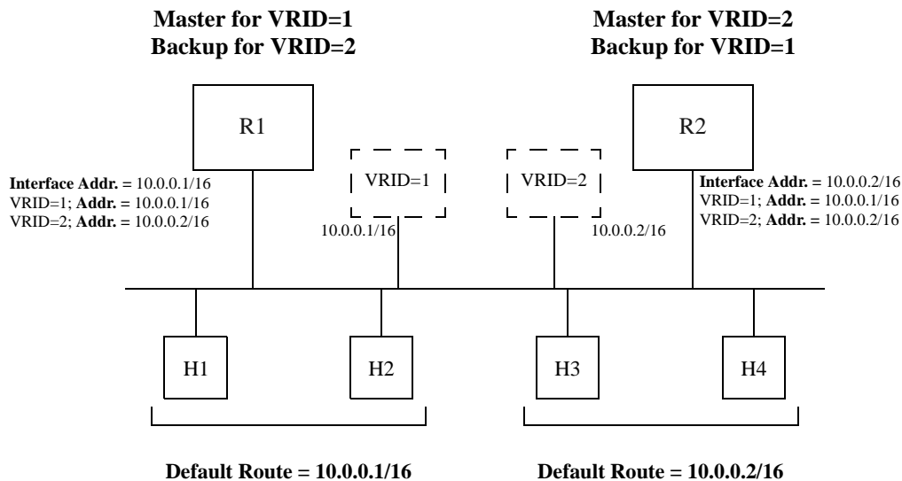
Figure 7. Symmetrical VRRP Configuration
