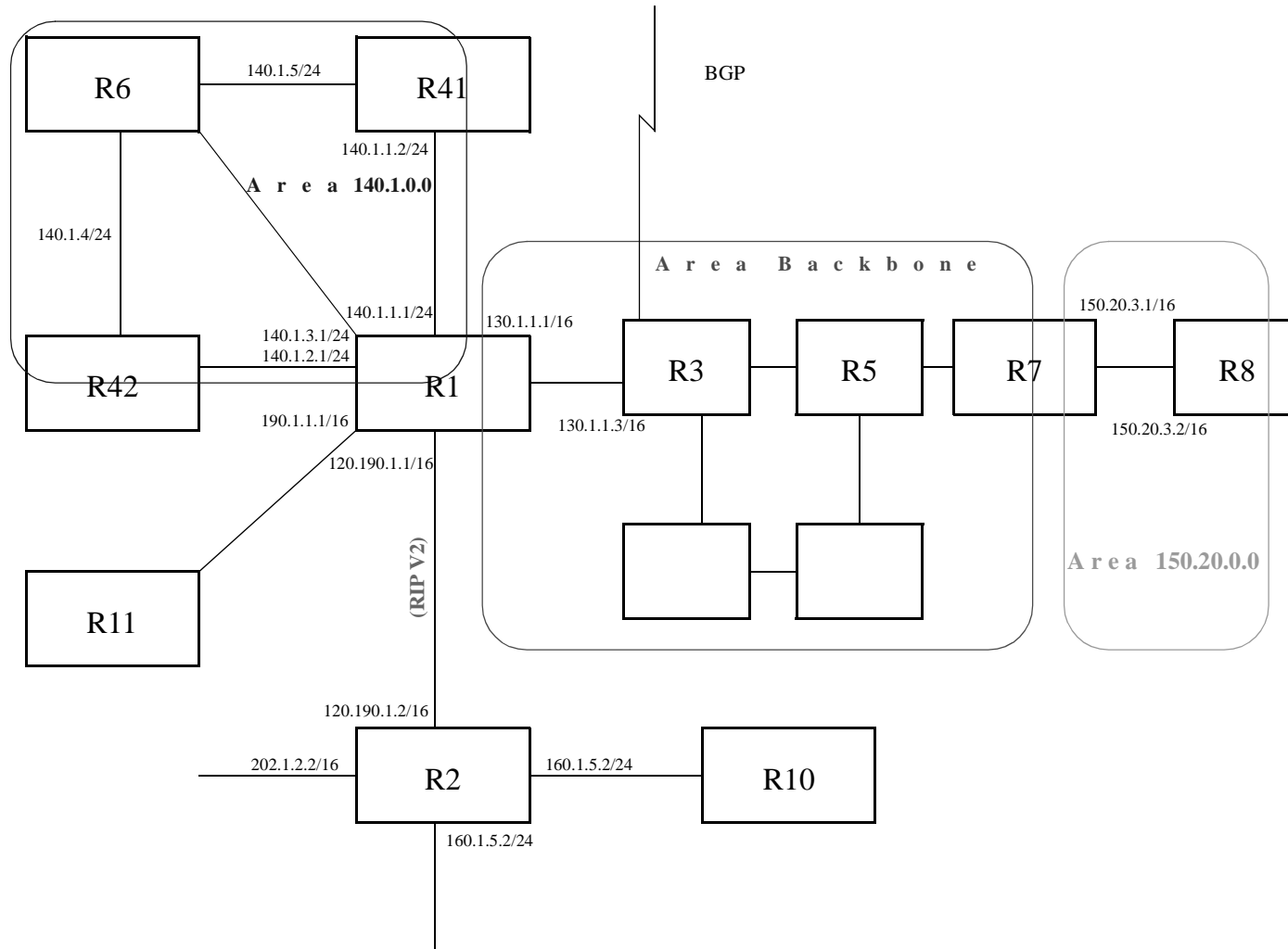
Figure 20. Exporting to OSPF
